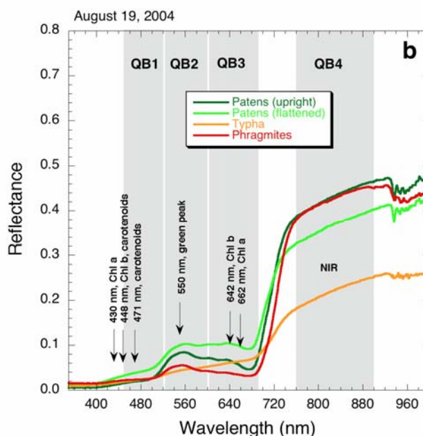
Fig. 4. Spectral reflectance of S. patens , Typha spp., and P. australis acquired through in situ radiometry, August 19, 2004.
